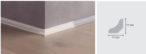
Hulkehl PGSCOTWHITE, 2400 × 17 × 17 mm – hvid PGSCOTPAINT, 2400 × 17 × 17 mm – kan males
